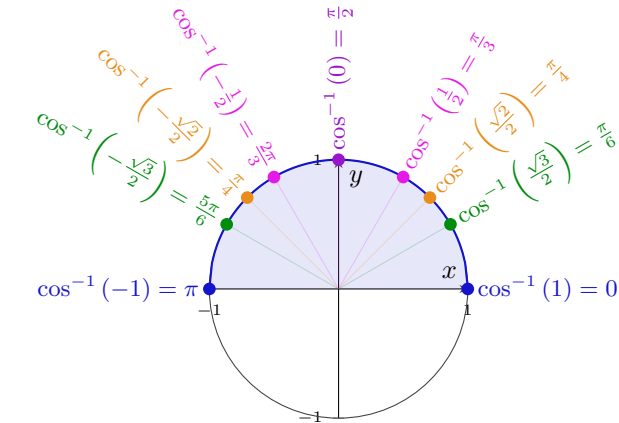
Figure 6.15: Unit Circle with Standard Inverse Co-sine Values
