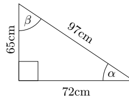
Figure 5.6: A right triangle
